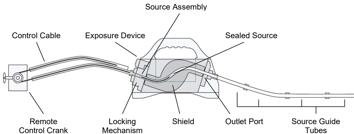
Figure 4. Sealed source in fully shielded position of radiographic exposure device
