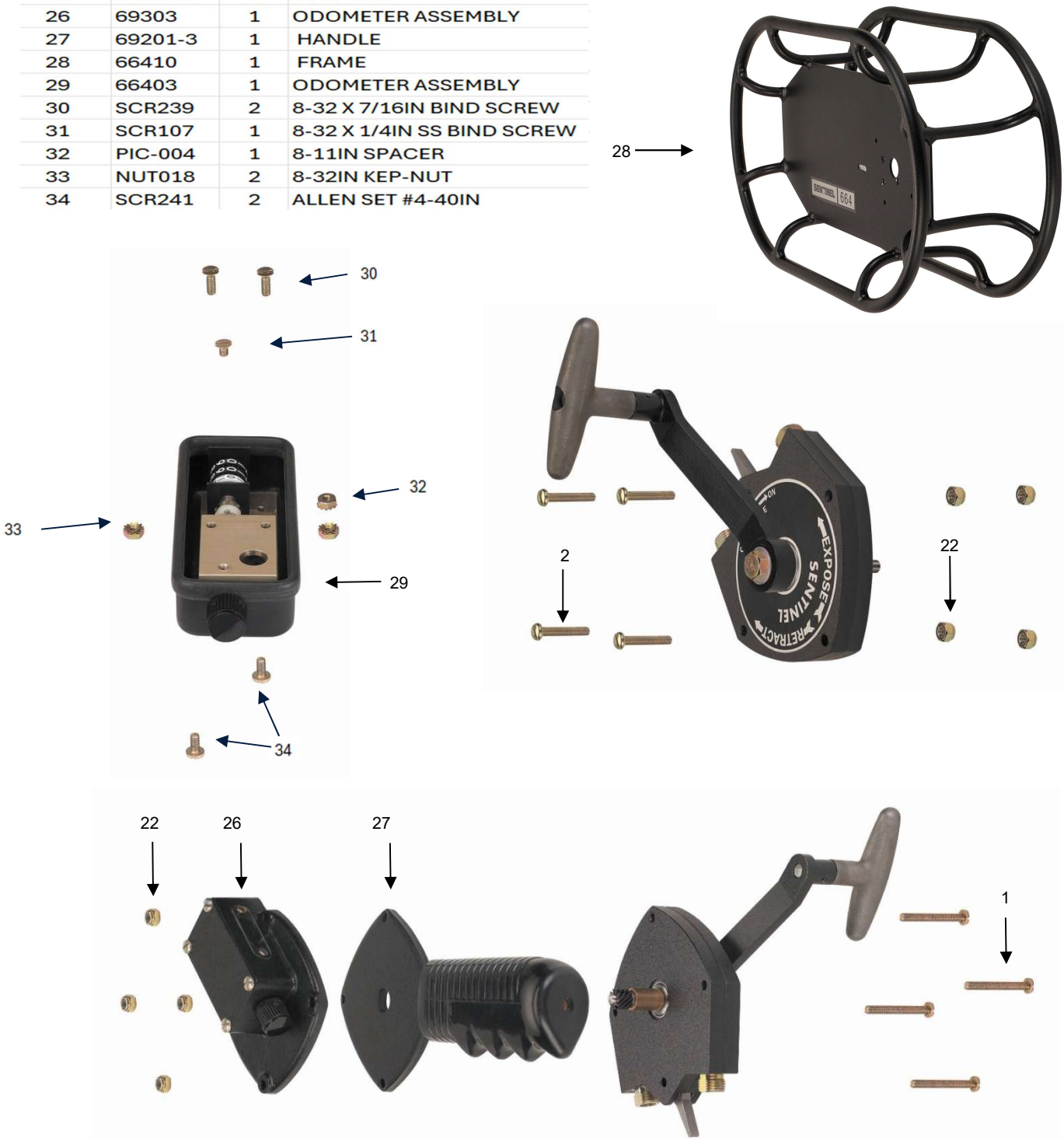
Figure 21. Reel and Reel Odometer (Model 664) & Hand Cranks (Model 692 and 693)
