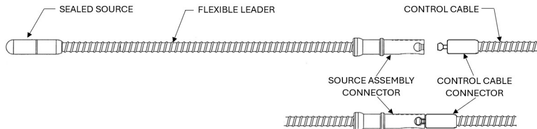
Figure 3. Source assembly and remote control cable connectors
