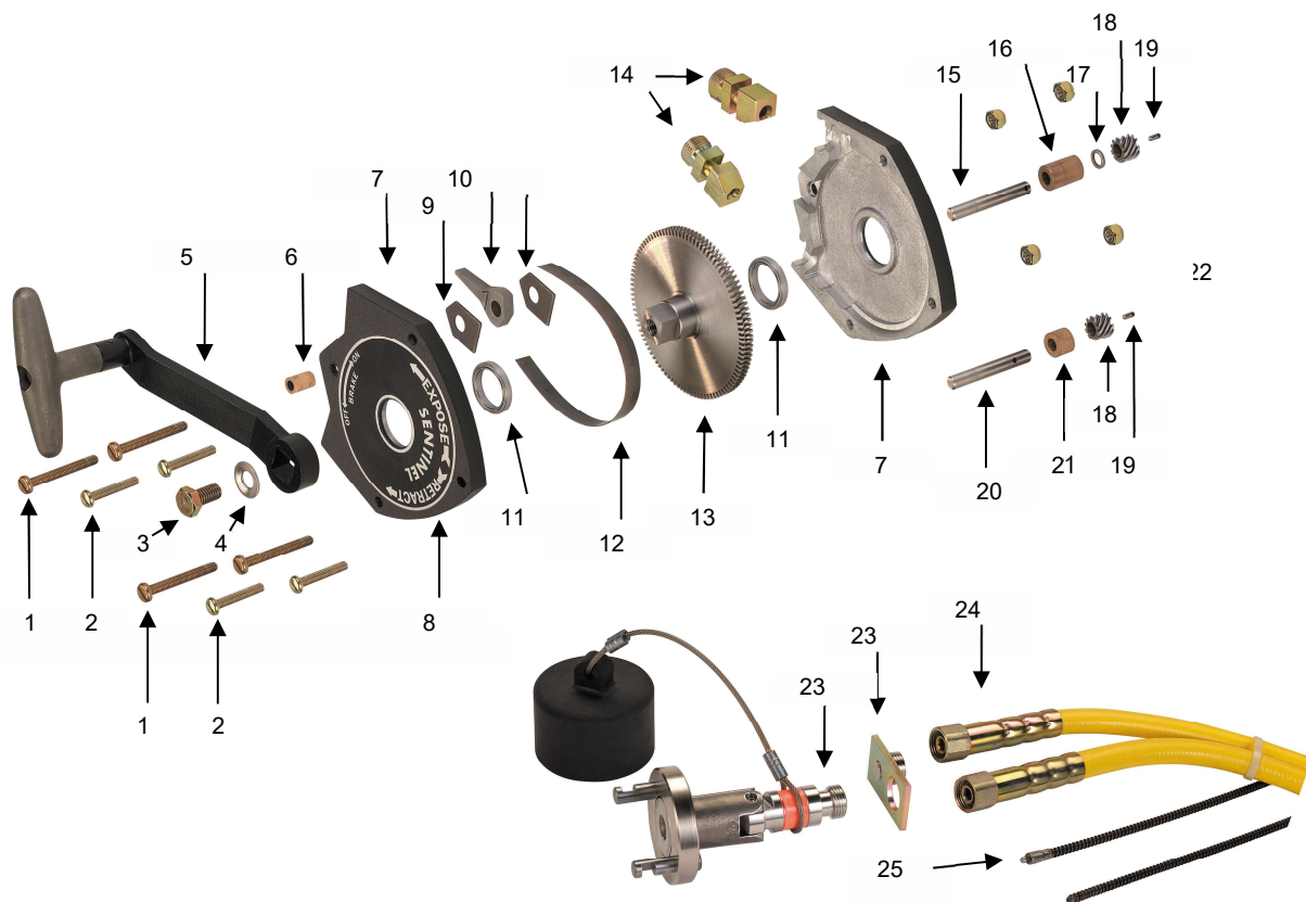
Figure 16. Remote Control Hand Crank Assemblies (Model 692, 693, and 664)
