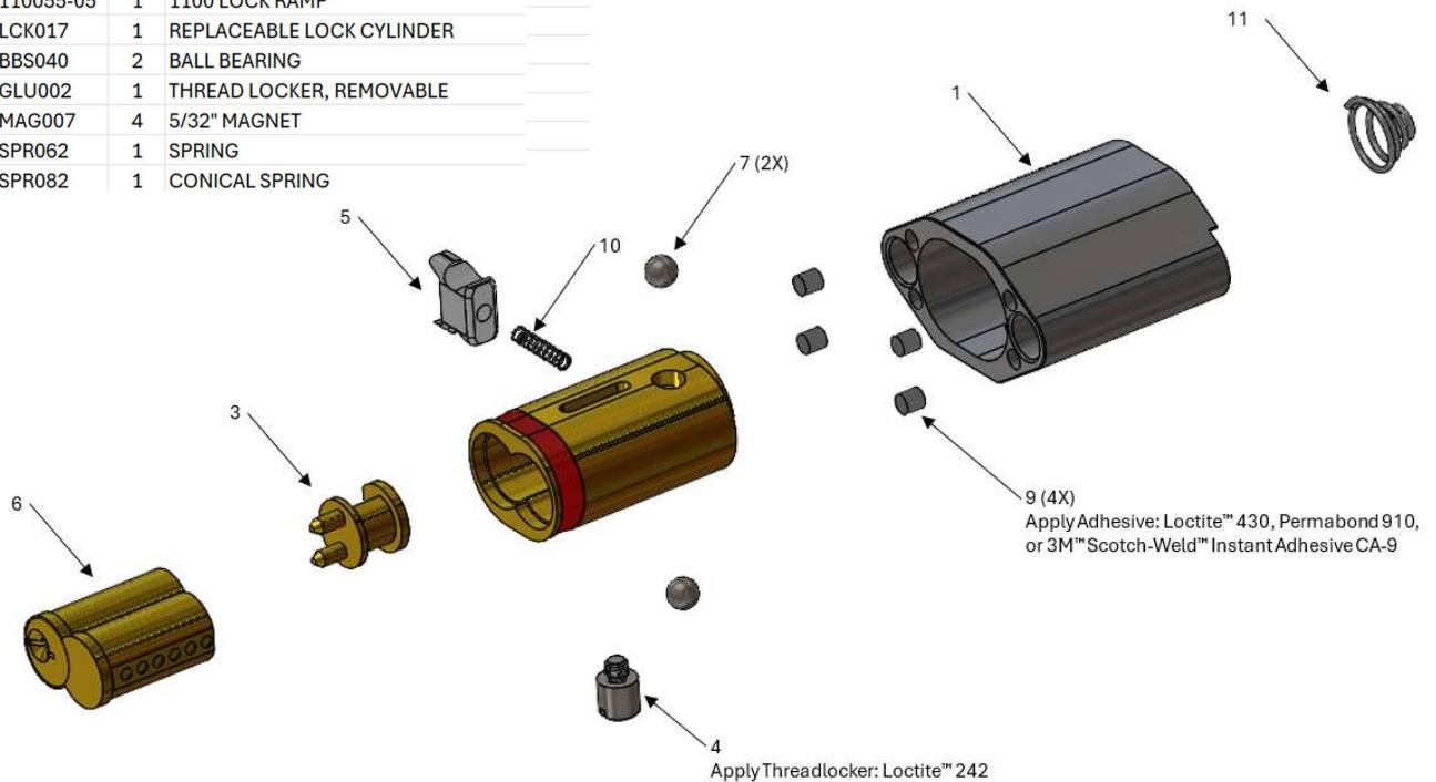
Figure 11. Lock Assembly
