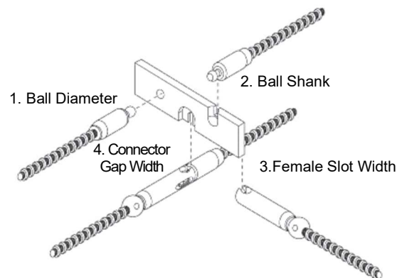
Figure 8. No-Go gauge tests
