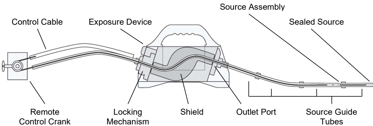
Figure 6. Sealed source in the exposure mode
