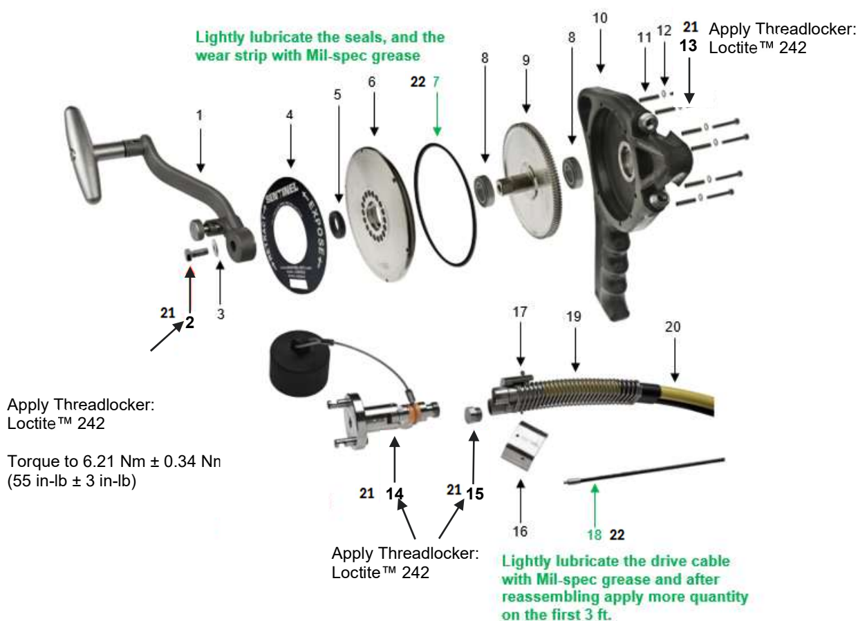
Figure 17. Remote Control Hand Crank Assemblies (Model 882 and 885 Series)
