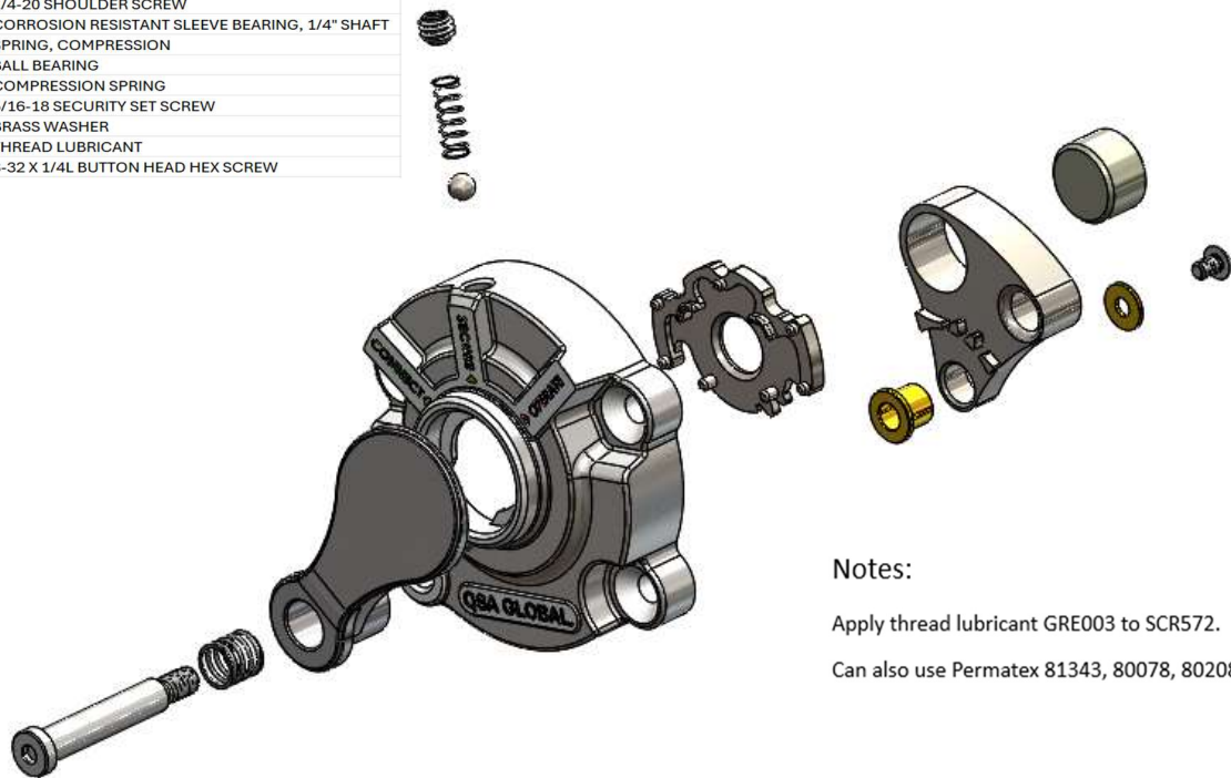
Figure 13. Front Plate Assembly
