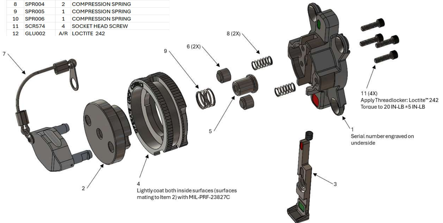
Figure 10. Rear Plate Assembly
