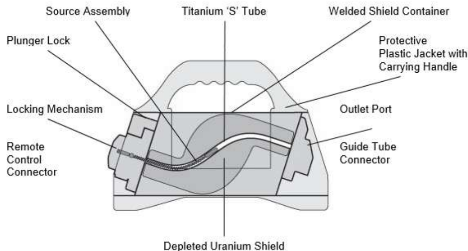
Figure 2. Model 1100 Major Components
