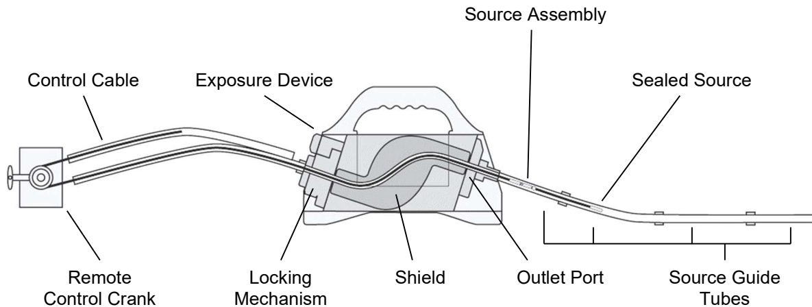
Figure 5. Sealed source in transit mode
