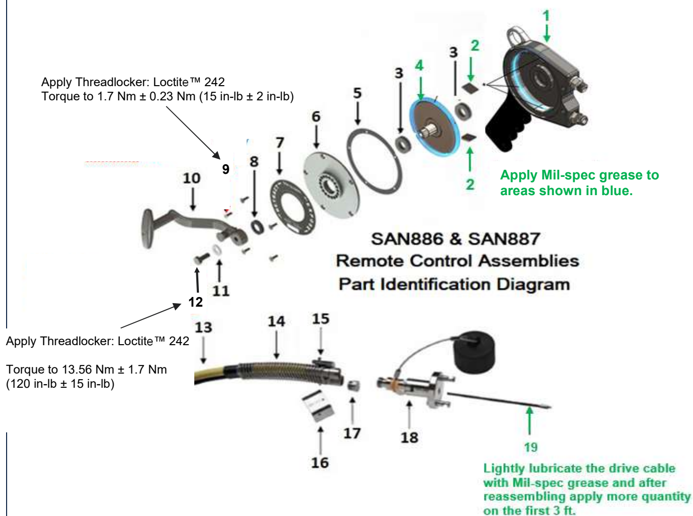
Figure 20. Remote Control Assemblies (SAN886 & SAN887)
